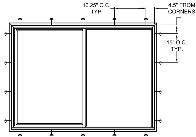
TYPICAL ELEVATION WITH FASTENER SPACING
